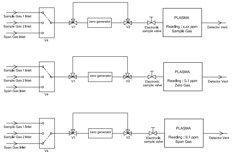
Figure 9: LD8000 with integrated zero calibrator & stream selector
