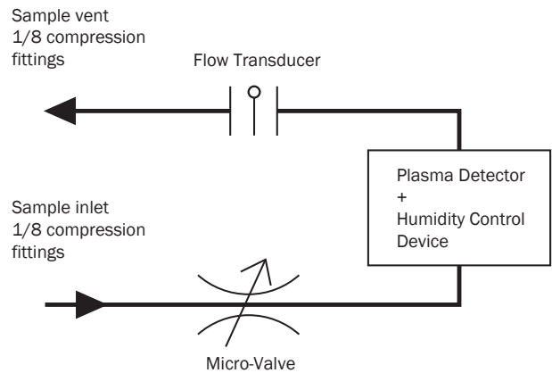
Figure 7: Flow path of the LD8000
