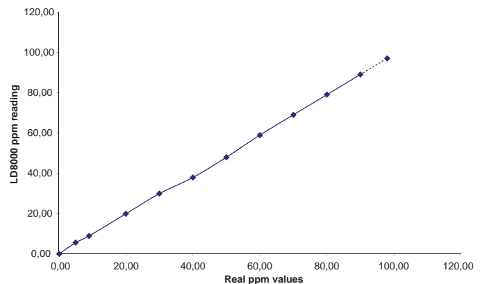
Figure 14: *LD8000 linearity on 0-100 ppm range
