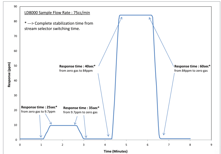
Figure 10: *LD8000 Reponse time
