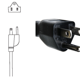
Plug Code "A" North America Plug
